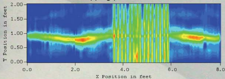
Mapping post tension cable and rebar
